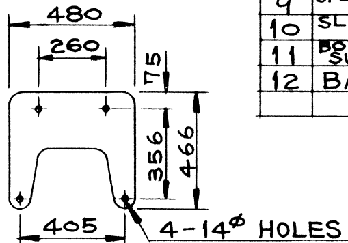
BASE DETAIL
